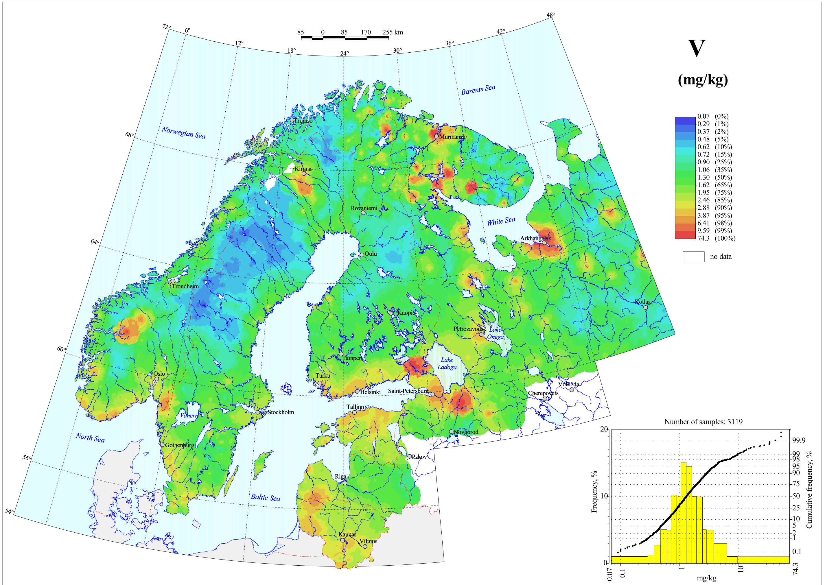
Vanadium in Terrestrial Moss, Total Content
